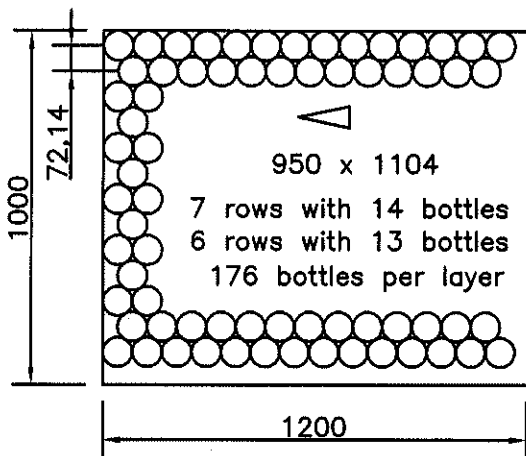
LAYOUT OF BOTTLES IN A PALLET
